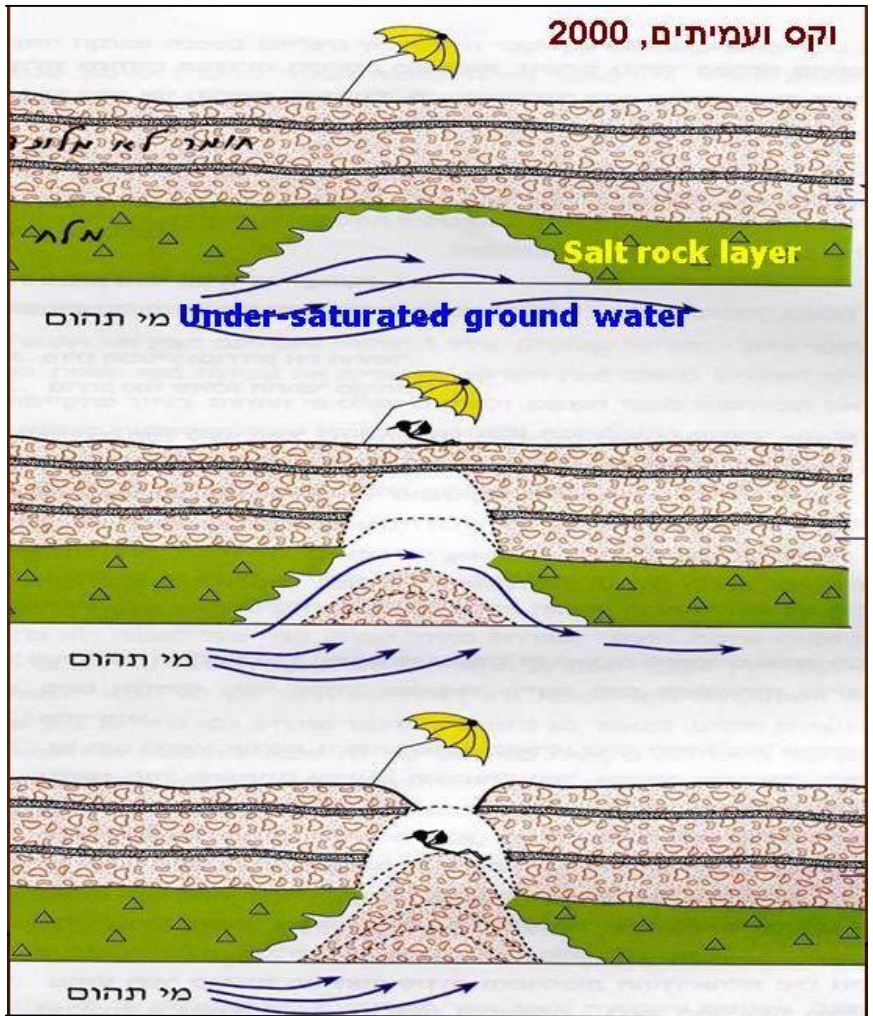
Hypothetic salt rock layer undergoing dissolution by under saturated ground water
