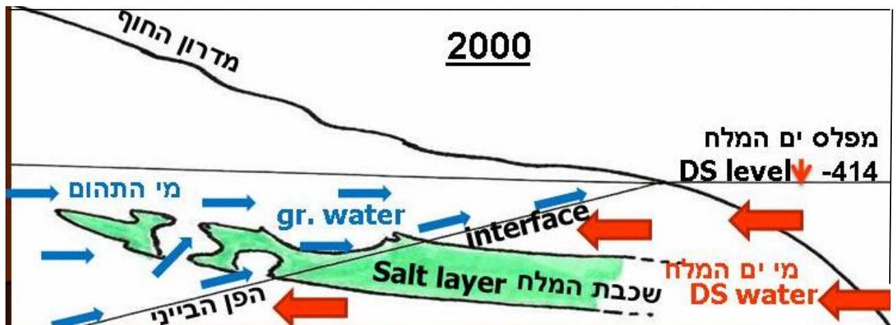
Exposure of the salt rock layer to dissolution by ground water following the sink of the interface, as a consequence of the drop in the level of the Dead Sea
